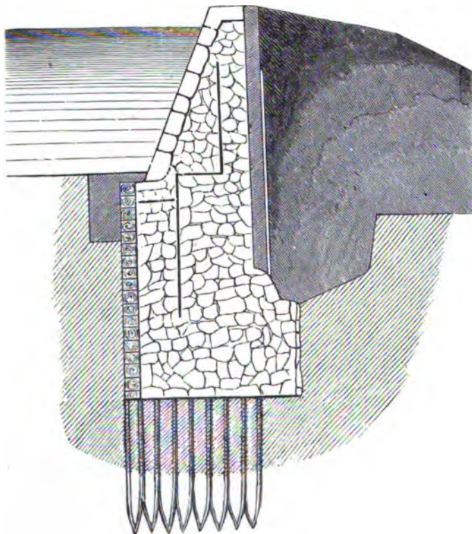
Fig. 234.—Masonry and earthen dam in Bavaria.
